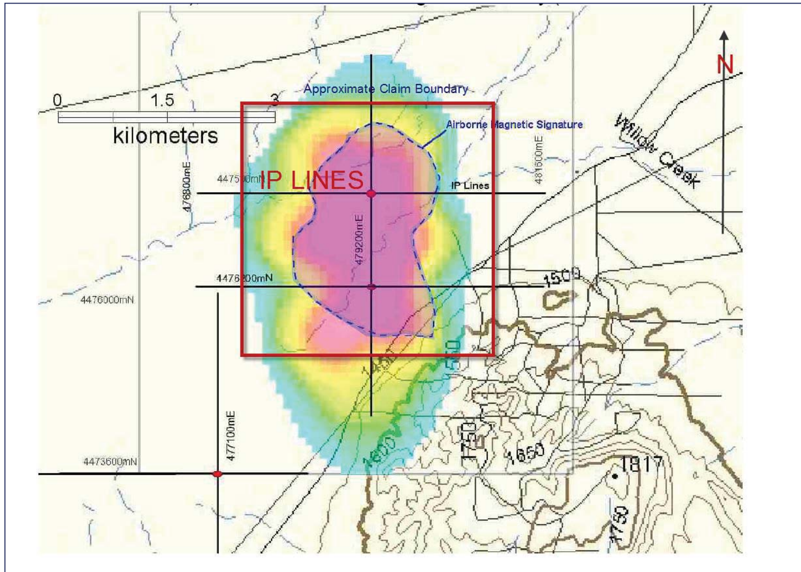
FIGURE 6. PLAN OF MAGNETIC AND IP ANOMALY AT ZPG (KENNECOTT 2002)
