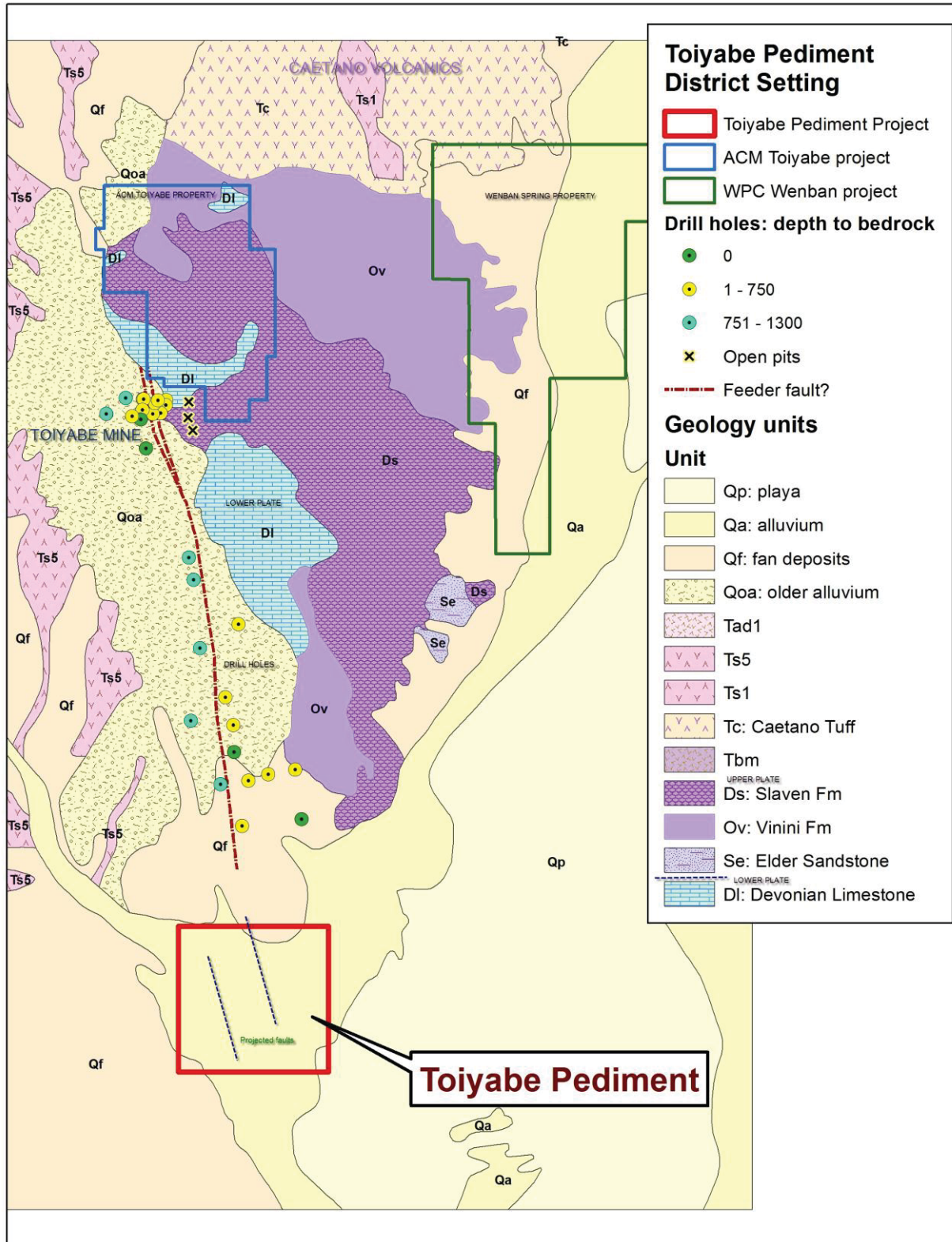
FIGURE 6. LOCAL GEOLOGY
