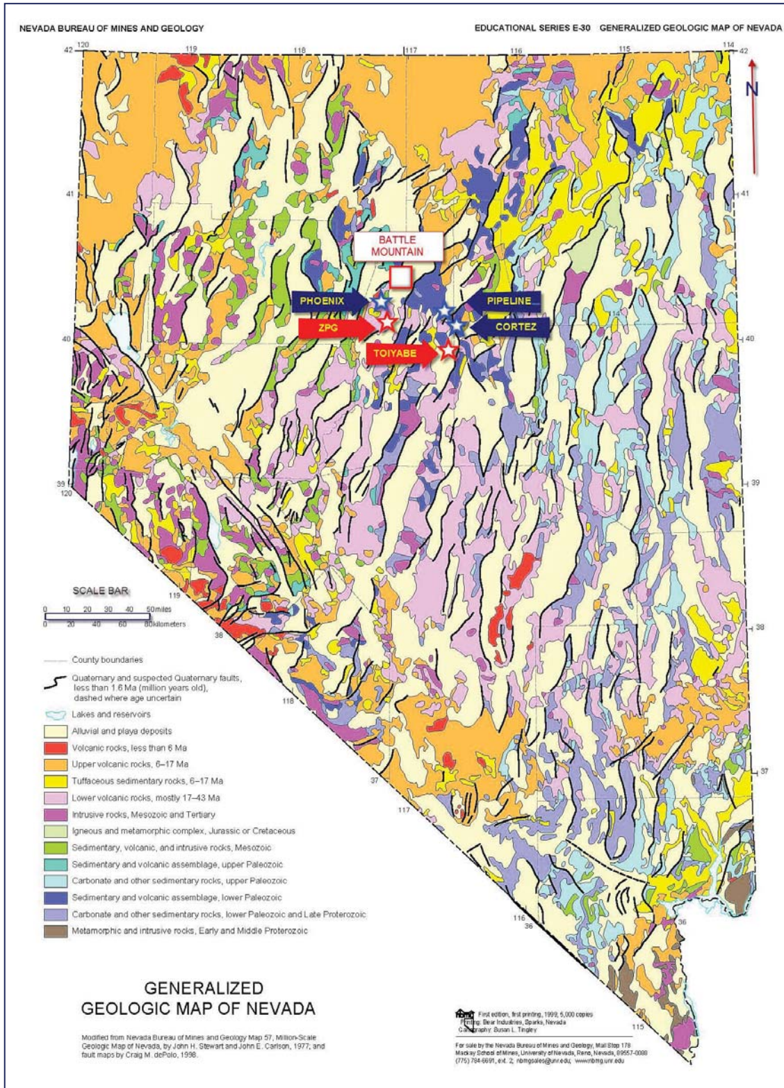
FIGURE 10. GENERALIZED GEOLOGY OF NEVADA
